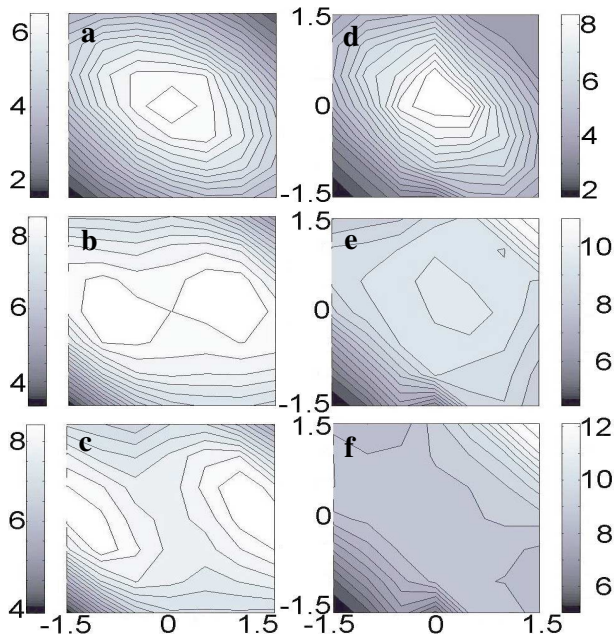
FIG. 3 (color online). Simulated constant-height FM-AFM images at three different heights of z_m = 3.10 , 2.40 , and 2.30 Å. The normalized frequency shifts ( fNm^{1/2} ) are indicated by the bar next to image. The left panel is for Si(001) tip: (a) at z_m = 3.10 Å, a single maximum; (b) at z_m = 2.40 Å, two maxima separated by \sim 1.5 Å; (c) at z_m = 2.30 Å, two most pronounced maxima separated by \sim 2.5 Å. The right panel is for Si(111) tip: at all distances, only one maximum with its position shifted from the center (d) to the upper-right corner (e),(f).
